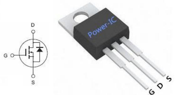
TO-220 Package
